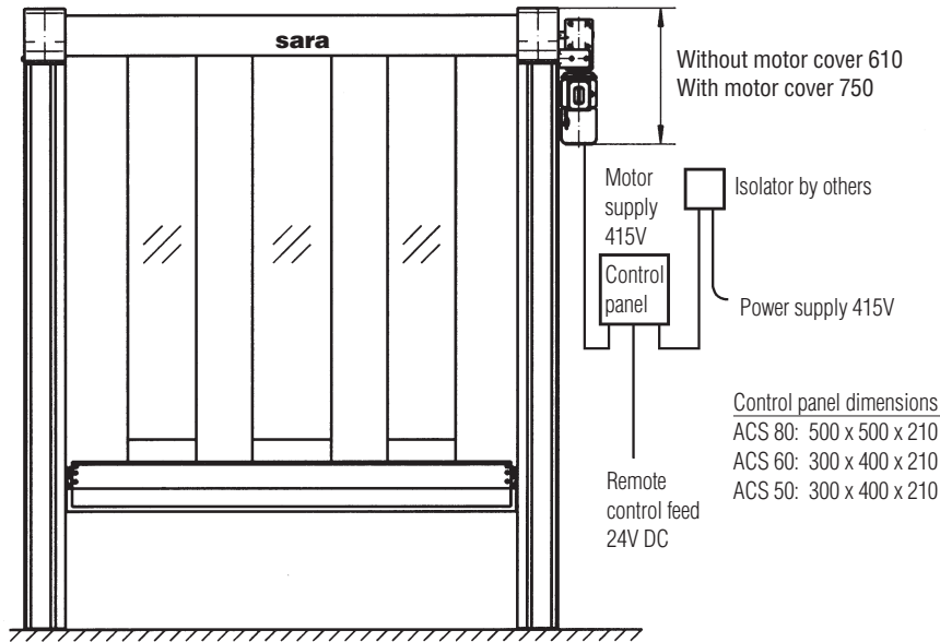
Elevation - direct drive
